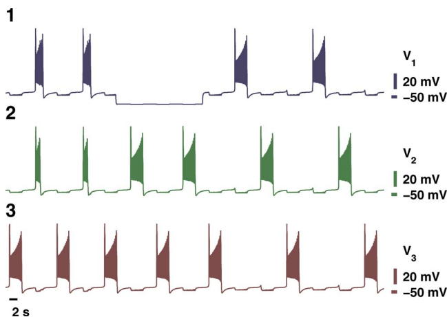
FIG. 8. (Color online) From winner to winnerless dynamics in the motif with asymmetrically weighted connection: g_{12}^{\text{in}}=1 , g_{21}^{\text{in}}=0.75 , g_{13}^{\text{in}}=0.75 , g_{31}^{\text{in}}=1.0 , g_{23}^{\text{in}}=1 , and g_{32}^{\text{in}}=0.75 , and V_{K2}^{\text{shift}}=-0.02 mV. The driving interneuron loses its superiority after the application of the external hyperpolarizing pulse to the driven interneuron. The original status can be restored as well.
