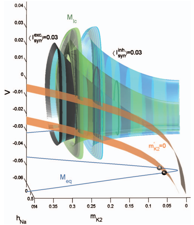
FIG. 1. (Color) Spiking M_{\text{lc}} and quiescent M_{\text{eq}} slow motion manifolds along with the slow nullcline m'=0 in the phase space of model (1) for V_{K2}^{\text{shift}} = -0.005 V (lower brown surface) and -0.024 V (upper). The spiking manifold M_{\text{lc}} is shown for three effective synaptic currents \langle I_{\text{syn}}^{\text{exc}} \rangle = 0.03 , \langle I_{\text{syn}}^{\text{inh}} \rangle = 0 , \langle I_{\text{syn}}^{\text{inh}} \rangle = 0.03 , respectively. Increasing V_{K2}^{\text{shift}} , or raising the inhibitory synaptic current \langle I_{\text{syn}}^{\text{inh}} \rangle hyperpolarizes the interneuron. The new stable equilibrium state at the intersection of the nullcline m'=0 with the low, hyperpolarized branch of M_{\text{eq}} corresponds to the locked-down state of the interneuron. In contrast, decreasing V_{K2}^{\text{shift}} , or raising \langle I_{\text{syn}}^{\text{exc}} \rangle brings both nullclines m'=0 and M_{\text{lc}} closer, thus slowing down the potassium current. This may further result in the emergence of a stable periodic orbit around M_{\text{lc}} corresponding to the tonic spiking activity of the interneuron.
