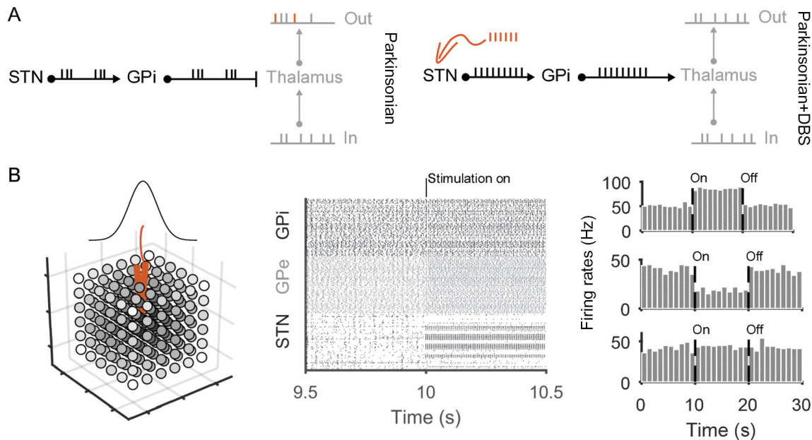
Figure 3 Model insights into the mechanisms of STN deep brain stimulation. 568 (A) Schematic of regularisation theory. 568 Left: models predict that, under parkinsonian conditions, the burst firing of GPI neurons, driven by STN burst firing, prevents the transmission of information through the thalamus. In this example, the thalamic output spike train is both missing spikes and produces additional spikes (orange) compared with the input. Right: when simulated high-frequency stimulation is applied to the STN (red spikes), the consequent regularisation of the GPI output restores transmission through the thalamus. (B) Mixture theory, after. 571 Left: network-scale models simulate a three-dimensional spread of current around the stimulating electrode (red) in STN, schematically illustrated here for a cube of STN neurons. Grey-scale shading is proportional to the magnitude of current received by each neuron from the central electrode (darker shading indicates more current). Middle: as a consequence, turning on the stimulation causes a mixed response in the STN, which leads in turn to a range of neuron firing patterns in GPI and GPe (raster plot: one row per neuron, each dot is one spike). Right: the network models predict that sustained high-frequency stimulation leads to a mixture of responses in GPI output, for which we show three example neurons: excited (top), inhibited (middle) and unaffected (bottom). The proportions of each response in the network model match those seen in therapeutic high-frequency stimulation in primates. 573 GPe, globus pallidus, external segment; GPI, globus pallidus, internal segment; STN, subthalamic nucleus.
