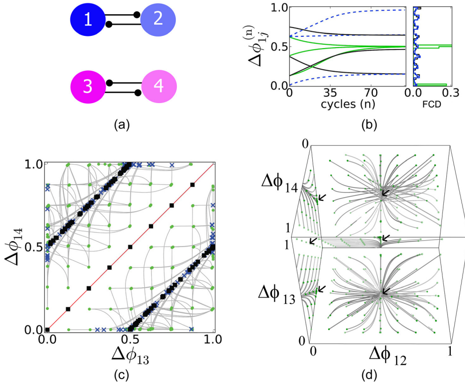
FIG. 5. (a) Dissected CPG made of uncoupled HCOs: g_{13}^{\text{inh}} = g_{24}^{\text{inh}} = 0 . (b) Phase-lag progressions (green, black, and blue curves for \Delta\phi_{12} , \Delta\phi_{13} , and \Delta\phi_{14} , resp.) indicating multiple phase-locked states, and the FCD of terminal phase-lags with two distinctive green peaks corresponding to in- and anti-phase states in HCO1 for g_{32}^{\text{inh}} = 5 \times 10^{-4} (1 + \delta_{ij}) , g_{41}^{\text{inh}} = 5 \times 10^{-4} . (c) 2D (\Delta\phi_{13}, \Delta\phi_{14}) -projection of the phase space of the map: green dots unmask the lattice of initial phases; blue crosses indicate the terminal points of (40 burst cycle long) trajectories on the line \Delta\phi_{14} = \Delta\phi_{13} + 1/2 \pmod{1} , corresponding to anti-phase bursting HCO2, and the (red) bisectrix corresponds to the in-phase bursting HCO1. Black squares indicate stagnation areas. (d) 3D return map revealing an attractor with \Delta\phi_{12} = 0.5 corresponding to anti-phase bursting in HCO1.
