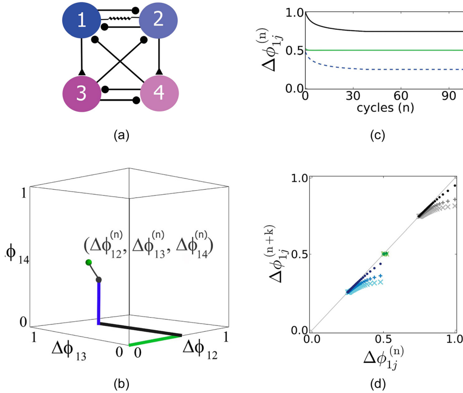
FIG. 2. (a) Schematic diagram of the swim CPG with two dedicated HCOs made of couples: Si1/2-L and Si1/2-R, and Si3-L and Si3-R. Dots, ●, solid triangles, ▲, and the resistor represent inhibitory, excitatory and electrical synapses of conductance strengths g_{ij}^{inh} , g_{ij}^{exc} , and g_{ij}^{elec} , respectively. (b) Phase-lag tuple (\Delta\phi_{12}^{(n)}, \Delta\phi_{13}^{(n)}, \Delta\phi_{14}^{(n)}) , is a phase point on the trajectory in the unit cube for 3D torus. Green sphere indicates an initial phase-lags tuple; green, black, and blue lines indicate n -th \Delta\phi_{12} , \Delta\phi_{13} , and \Delta\phi_{14} coordinates of the trajectory, where n varies from 0 to 100 along the depicted trajectory. (c) Evolutions of the phase-lags, \Delta\phi_{12}^{(n)} (green), \Delta\phi_{13}^{(n)} (black), and \Delta\phi_{14}^{(n)} (blue) plotted against the burst cycle, n . (d) 1D Poincaré maps of degrees: k=1 (dots), k=5 (small dark pluses), k=10 (large light crosses) for the (color-coded) phase-lags showing the convergence to fixed points on the 45°-line: \Delta\phi_{12}^* = 1/2 , \Delta\phi_{13}^* = 3/4 , and \Delta\phi_{14}^* = 1/4 for specific g_{12}^{inh} = g_{21}^{inh} = 2.25g_{max} , g^{elec} = 0.25g_{max} , and nominal conductances g = g_{max} = 2.5 \times 10^{-3} .
