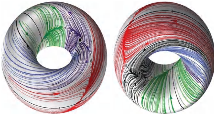
Figure 5. Poincaré return maps depicted on the torus. The return maps for the phase lags \{\Delta\phi_{21}^{(n)}, \Delta\phi_{31}^{(n)}\} between homogeneous cells at 50% DC correspond to trajectories on a 2D torus [0,1) \times [0,1) . Different colors denote attractor basins of several FPs corresponding to phase locked states of distinct bursting rhythms. doi:10.1371/journal.pone.0092918.g005
