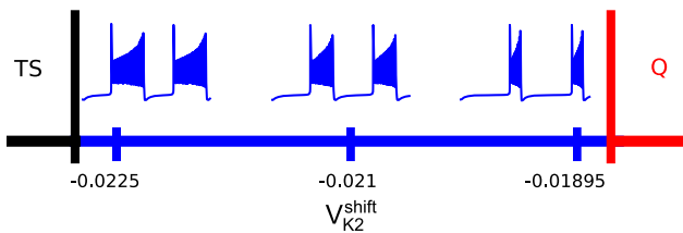
Figure 2. Schematic showing regimes and how burst duration changes as the bifurcation parameter, V_{K2}^{shift} is varied. Burst duration increases as V_{K2}^{shift} approaches the boundary of the tonic spiking (TS) state, and decreases towards the boundary of hyperpolarized quiescence (Q). The post-synaptic cell on the network can temporarily cross either boundary when excited or inhibited by synaptic currents from pre-synaptic neurons.
